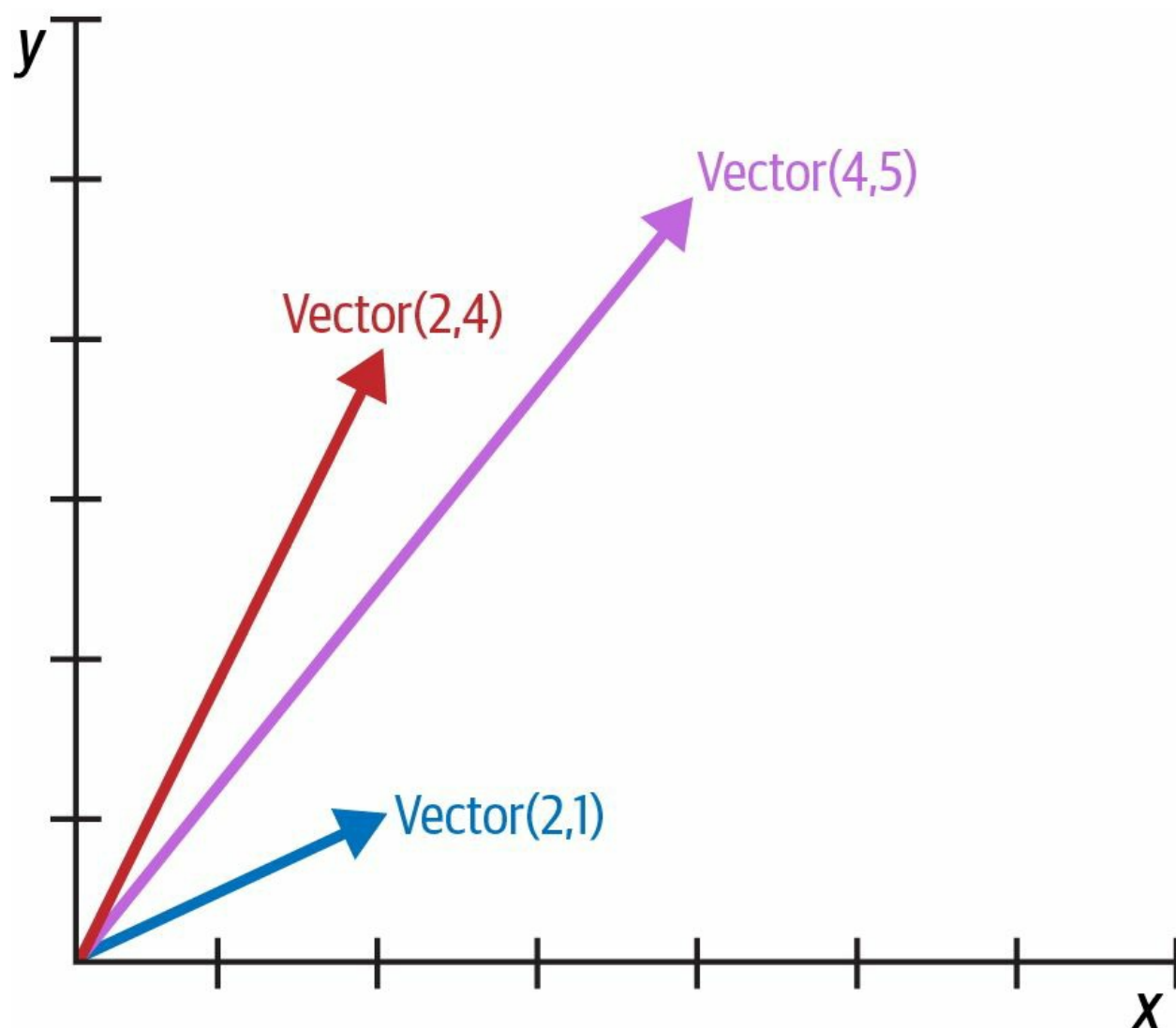
图 1-1：二维向量加法图示： \text{Vector}(2, 4) + \text{Vector}(2, 1) = \text{Vector}(4, 5)
